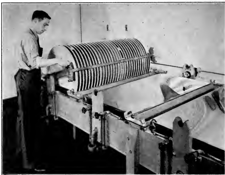
FIG. 2. Showing the manual transfer of a drum from tray to tray by means of the lever mechanism on the drum.
